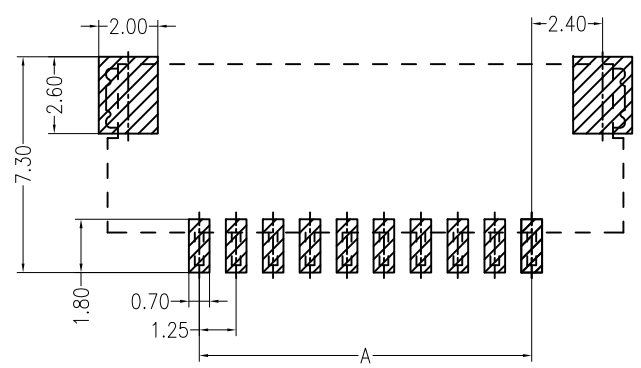
PCB LAYOUT(Tolerance: \pm 0.05 )
