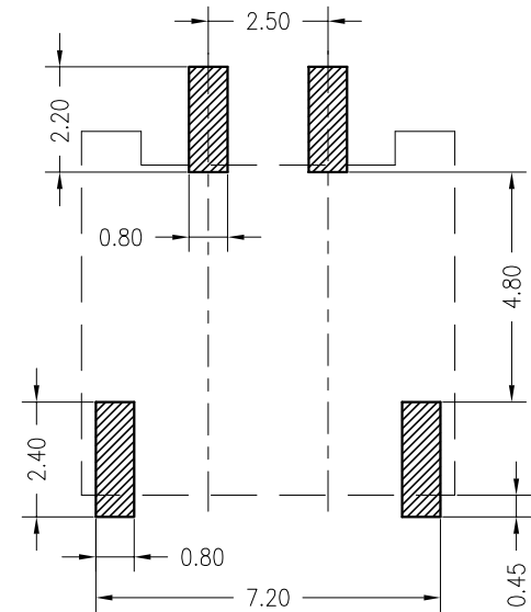
Board Layout
