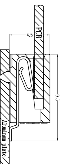
Assembly Layout
