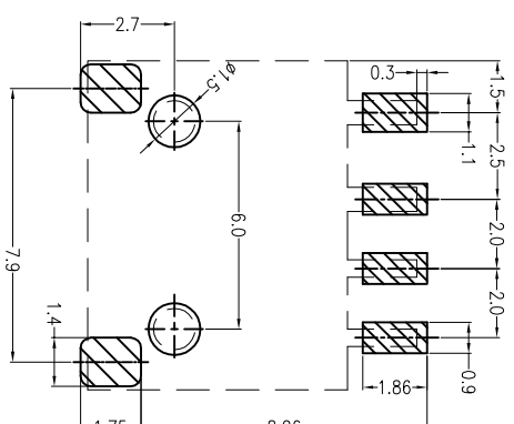
Board Layout
