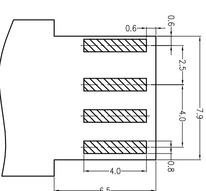
Mating Aluminum plate detail
