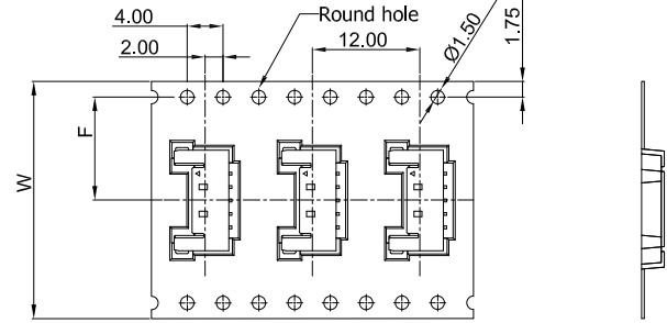
08~12 CONTACTS
