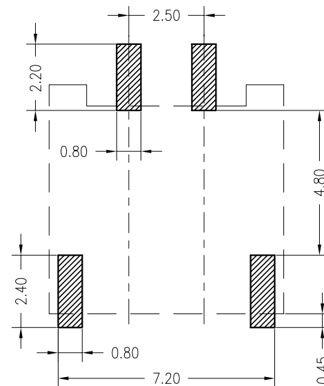
Board Layout
